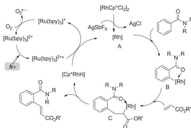
Scheme 1. Working hypothesis for the combined rhodium- and photoredox-catalyzed C–H functionalization. Cp* = C 5 Me 5 .
