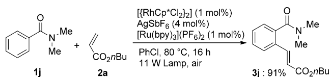
Scheme 2. Control reactions to exclude internal oxidants.
